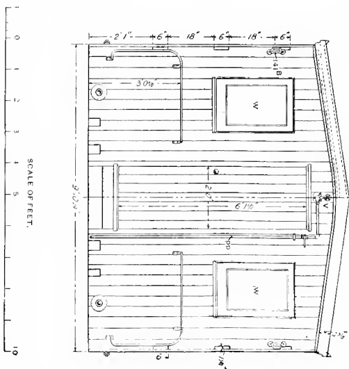
Fig. 270. End Elevation.
